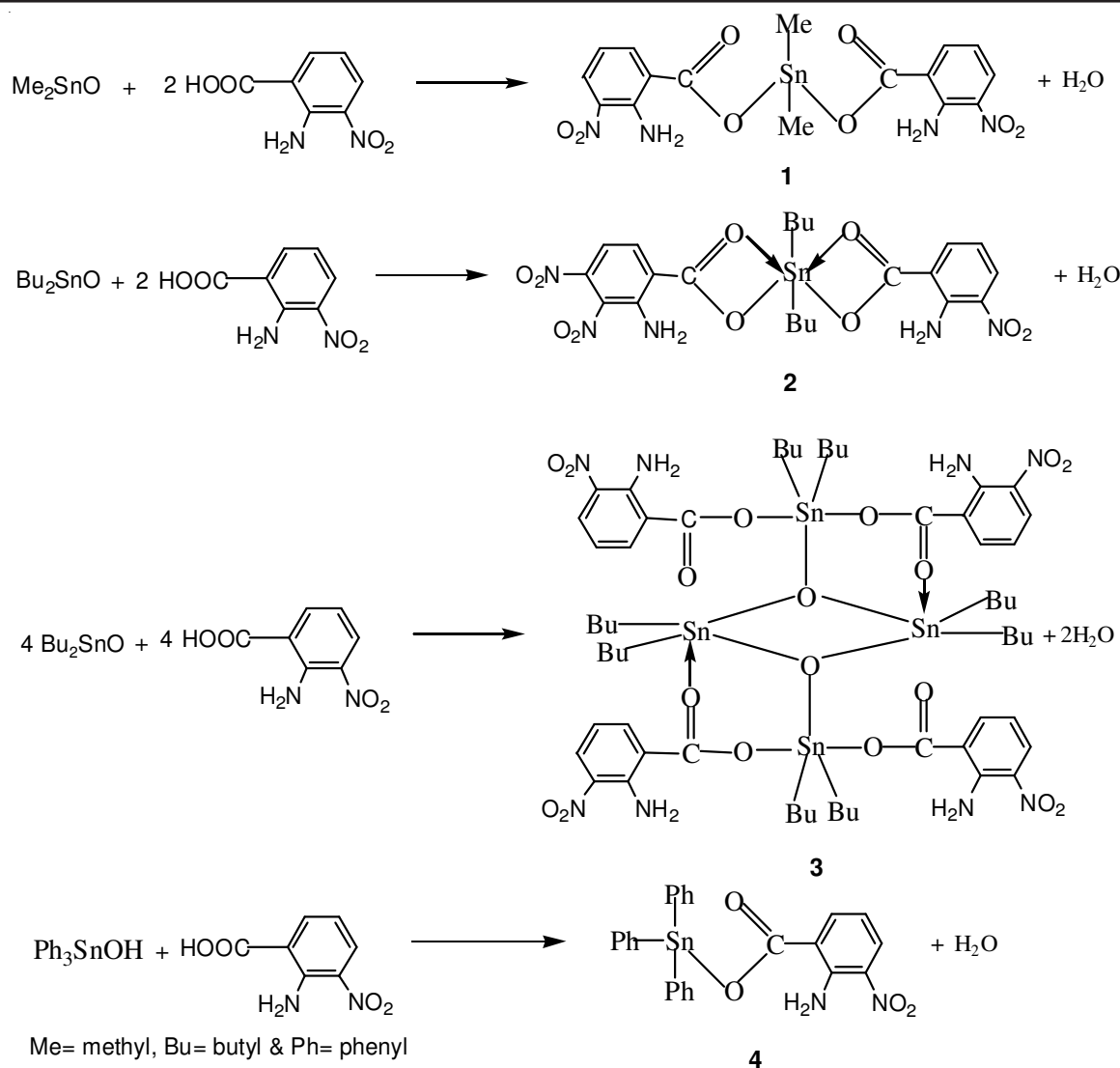
Fig. 1. Proposed structure of complexes 1-4
