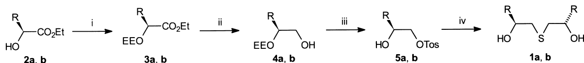
Scheme 2. Synthesis of chiral thiodiglycoles 1a ( \text{R}=\text{Me} ) and 1b ( \text{R}=\text{Ph} ); reagents, conditions, and yields: (i) \text{H}_2\text{C}=\text{CHOEt} , cat. \text{TosOH}\cdot\text{H}_2\text{O} , 3a : 98%, 3b : 100%; (ii) \text{LiAlH}_4 , \text{Et}_2\text{O} , 4a : 95%, 4b : 98%; (iii) 1. \text{TosCl} , pyridine, 2. \text{HCl}-\text{H}_2\text{O} , 5a : 91%, 5b : 94%; (iv) \text{Na}_2\text{S} , acetone, 70^\circ\text{C} , 1a : 88%, 1b : 82%; \text{EE}=\text{EtO}(\text{Me})\text{CH} , \text{Tos}=\text{pMeC}_6\text{H}_4\text{SO}_2
