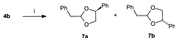
Scheme 4. Formation of dioxolane derivatives 7a and 7b from 4b ; reagents, conditions, and yields: (i) 0.5 equiv. (CF 3 SO 2 ) 2 O, 1.0 equiv. pyridine, THF, –30°C, 45 min, 7a : 19%, 7b : 17%
