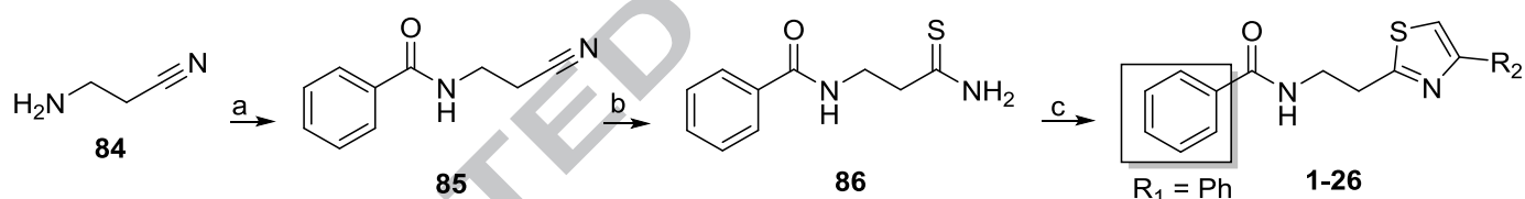
Scheme 1. Synthesis of compounds 1–26 . Reagents and conditions: a) benzoyl chloride, \text{Et}_3\text{N} , THF, -5\text{ }^\circ\text{C} to rt, overnight; b) \text{NaHS}\cdot x\text{H}_2\text{O} , \text{MgCl}_2 , 15-crown-5, DMF, rt; c) appropriate 1-aryl-2-bromoethanone, EtOH, reflux or rt. Structures 1–26 are defined in Table 1.
