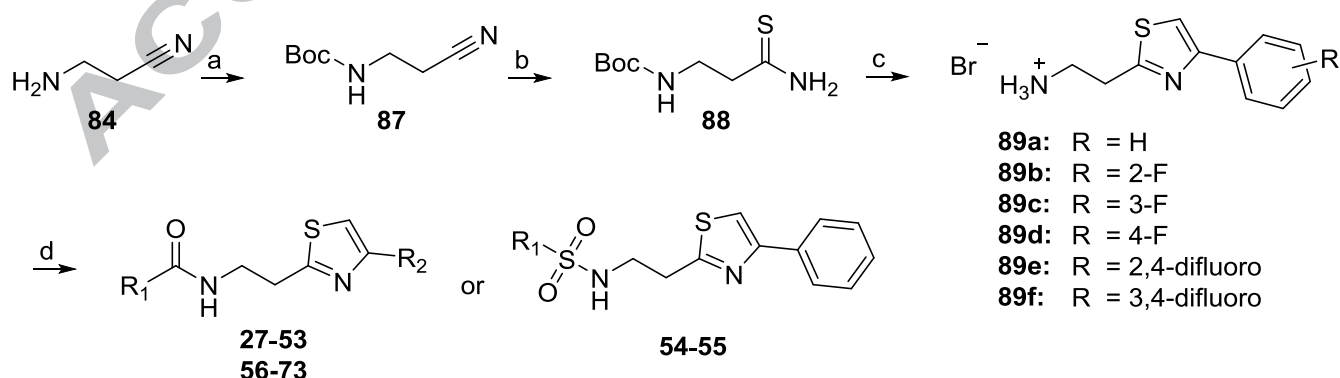
Scheme 2. Synthesis of compounds 27–73 . Reagents and conditions: a) \text{Boc}_2\text{O} , Montmorillonite K-10; b) \text{NaHS}\cdot x\text{H}_2\text{O} , \text{MgCl}_2 , 15-crown-5-, DMF, rt; c) appropriate 1-aryl-2-bromoethanone, EtOH, reflux; d) appropriate carbonyl or sulfonyl chloride, anhydride, or isocyanate, \text{Et}_3\text{N} (or DIEA), THF (or DCM). Structures 27–55 and 56–73 are defined in Tables 2 and 3, respectively.
