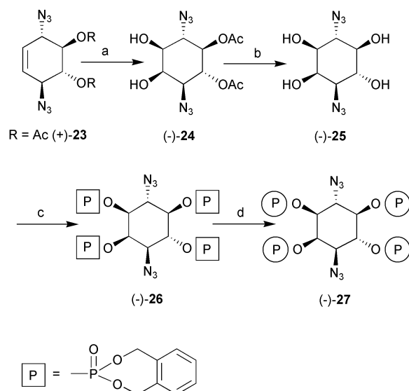
Scheme 7 Reagents and conditions: (a) RuCl 3 , NaIO 4 , CH 3 CN (99%). (b) NaOMe, MeOH (99%). (c) (1,5-dihydro-2,4,3-benzodioxaphosphin-3-yl)diethylamine, 1 H -tetrazole, CH 3 CN, then m -CPBA (45%). (d) CH 2 Cl 2 , TMSBr (90%).
