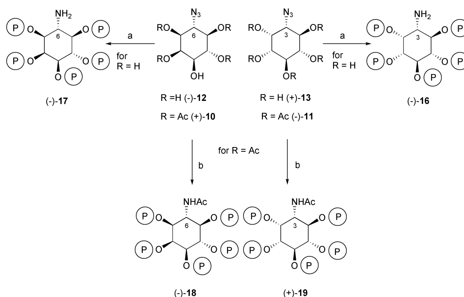
Scheme 4 Reagents and conditions: (a) 1, (1,5-dihydro-2,4,3-benzodioxaphosphin-3-yl)diethylamine, 1 H -tetrazole, \text{CH}_3\text{CN} , then m -CPBA (51%). 2, Pd/C, \text{H}_2 ethanol–water (90%). (b) 1, Pd/C, \text{H}_2 , methanol (80%). 2, \text{Ac}_2\text{O} , pyridine (99%). 3, NaOMe, MeOH (80%). 4, (1,5-dihydro-2,4,3-benzodioxaphosphin-3-yl)diethylamine, 1 H -tetrazole, \text{CH}_3\text{CN} , then m -CPBA (43%). 5, Pd/C, \text{H}_2 ethanol–water (80%).
