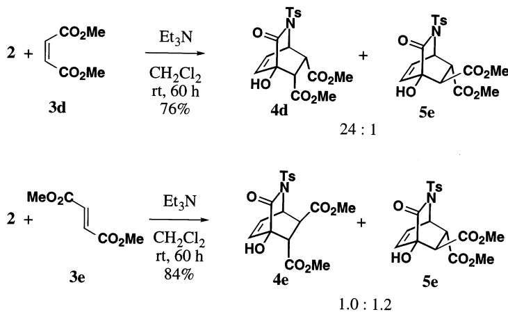
Scheme 2. Stereospecific base-catalyzed DA reaction
