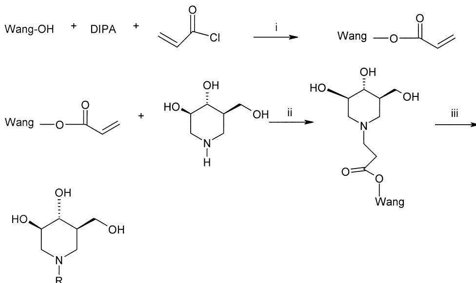
Scheme 5. Solid phase synthesis of N -substituted Isifagomine derivatives: (i) \text{CH}_2\text{Cl}_2 , 7H, rt; (ii) DMF, 22 h, rt, wash; (iii) (a) \text{R-Hal} , DMF, 24 h, rt (b) DIPEA, DMF, 24 h, rt.
