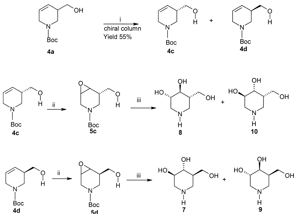
Scheme 3. Synthetic pathway to four stereoisomers of Isofagomine: (i) Chiracel OD or chiralpack AS, eluent \text{Pr}^i\text{OH} /heptane (1/99); (ii) MCPBA, \text{CH}_2\text{Cl}_2 , rt; (iii) KOH (10%).
