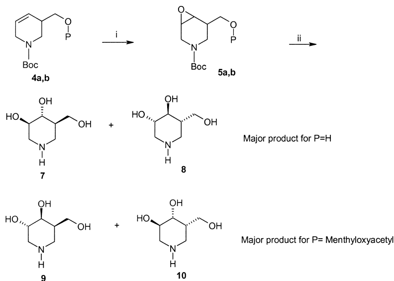
Scheme 2. Synthetic pathway to enantiomeric mixtures of Isogagomine: (a) P=H; (b) P=(−)-menthylxyacetyl; (i) MCPBA, CH 2 Cl 2 , rt; (ii) (a) KOH (10%) reflux; (b) purification on chiral plate (Merchery Nagel), eluent Pr i OH/25% NH 3 (3/1); (c) separation on HPLC, Merck LiChrosorb NH 2 , eluent 70% CH 3 CN aq; identification by MS and NMR.
