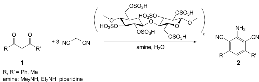
Scheme 1. Synthesis of 2,6-dicyano-3,5-disubstituted anilines 2a – c
