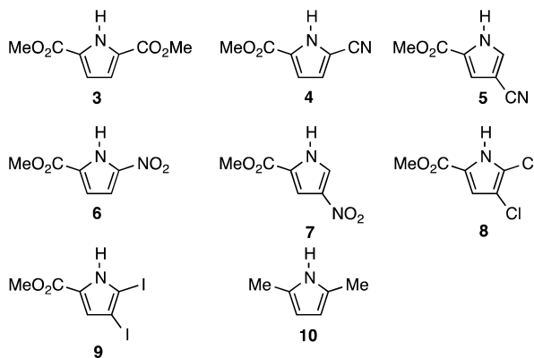
Figure 1. Starting monopyrroles.
