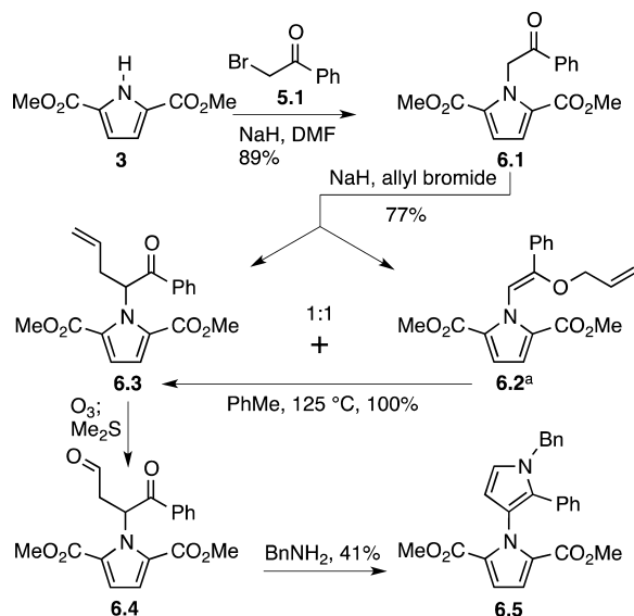
Scheme 6. Formation of 6.5
