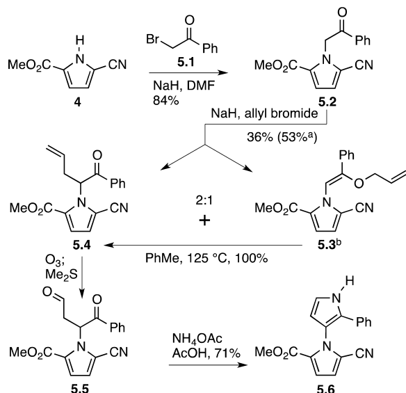
Scheme 5. Formation of 5.6
