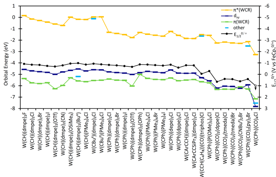
Figure 2. Oxidation potentials and calculated \pi^*(W\equiv CR) , d_{xy} , and \pi(W\equiv CR) orbital energies of W(CR)L_nL'_{4-n}X complexes (see Table 1 and Table S2 in the Supporting Information). Orbitals labeled “other” are indicated for compounds with additional orbitals in this energy space. The open circle for W(CPh)(CO)_4Cl represents the lower limit of the oxidation potential for W(CCCPh)(CO)_4Cl .
