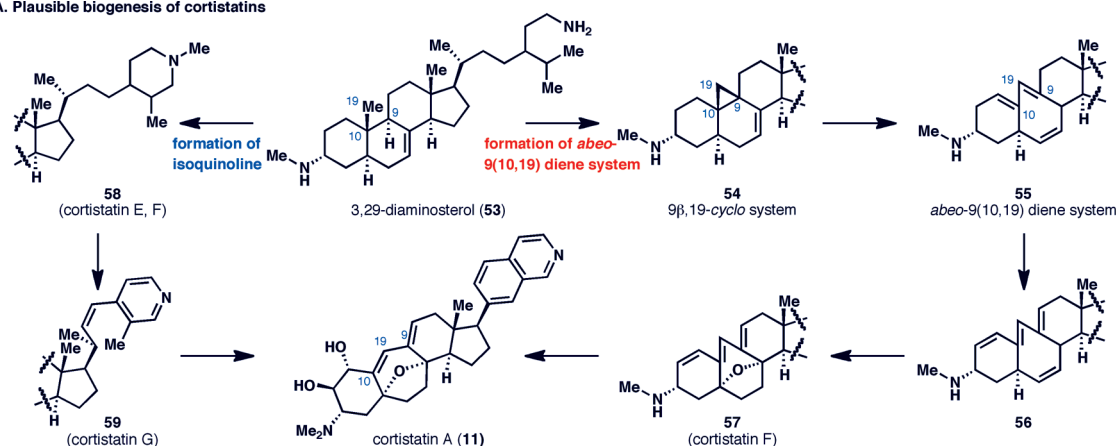
Scheme 9. Key Considerations and Historical Context for the B-Ring Expansion
