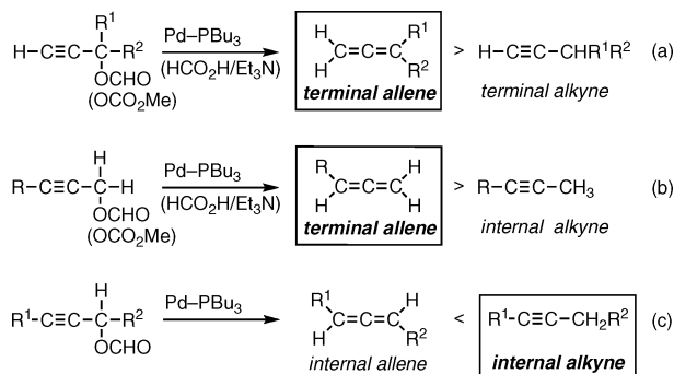
Scheme 1. Decarboxylative Hydrogenolysis of Propargylic Formates using a Pd-PBu 3 Catalyst System
