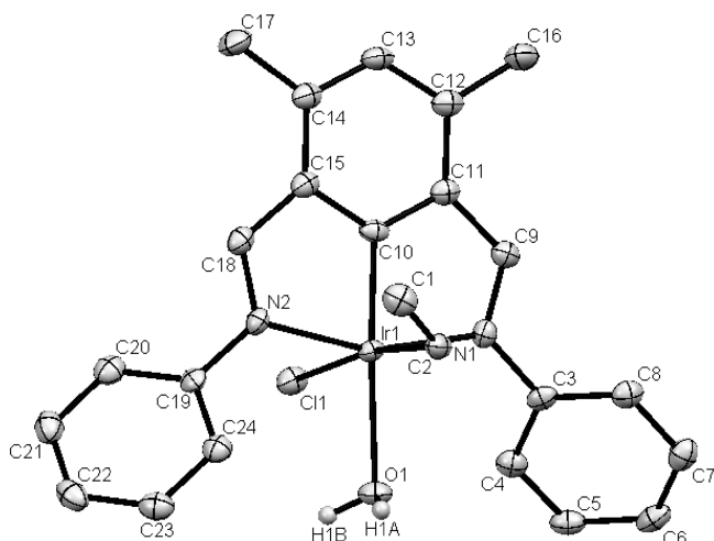
Figure 1. ORTEP diagram of (NCN)Ir(CH 2 CH 3 )(Cl)(OH 2 ) (3).
