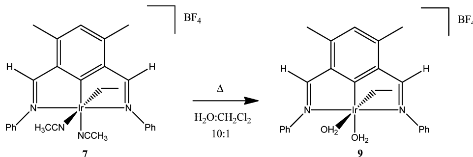
Scheme 10. Synthetic Route to [(\text{NCN})\text{Ir}(\text{CH}_2\text{CH}_3)(\text{OH}_2)_2][\text{BF}_4] (9)
