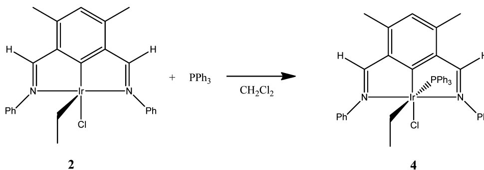
Scheme 5. Synthetic Route to (NCN)Ir(CH 2 CH 3 )(Cl)(PPh 3 ) (4)
