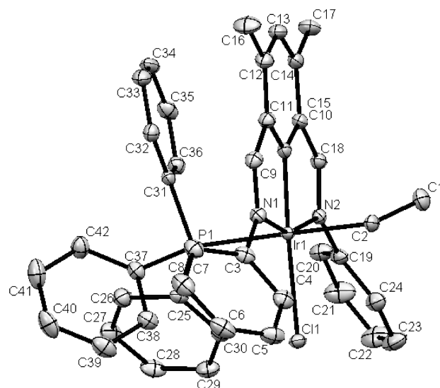
Figure 2. ORTEP of (NCN)Ir(CH 2 CH 3 )(Cl)(PPh 3 ) (4).
