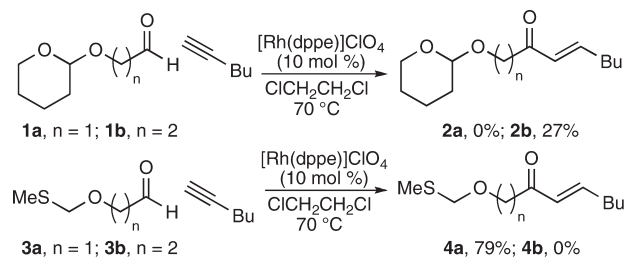
Scheme 1. O,O - and O,S -Acetals in Alkyne Hydroacylation
