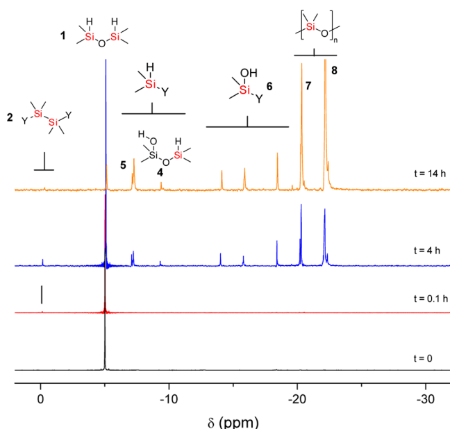
Figure 3. ^{29}\text{Si} NMR of the crude reaction mixture of \text{Ph}_3\text{PO} reduction by \text{TMDS}/\text{Ti}(\text{OiPr})_4 .
