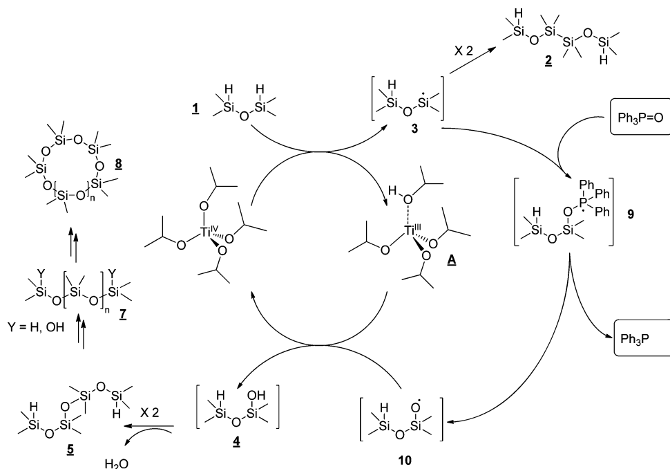
Scheme 2. Proposed Mechanism of \text{Ti}(\text{OiPr})_4 -Catalyzed Reduction of Triphenylphosphine Oxide by Hydrosiloxanes a
