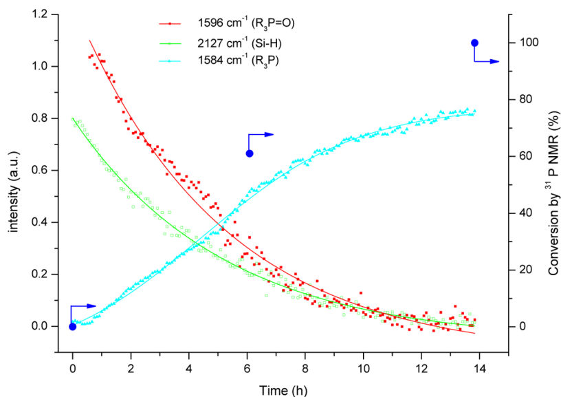
Figure 4. Monitoring of \text{Ph}_3\text{PO} reduction on a 100 g scale using Raman spectroscopy. Experimental conditions: \text{TMDS} (Si–H/P=O = 2.1), \text{Ti}(\text{OiPr})_4 10% cat., \text{Na}_2\text{SO}_4 (10 wt %), cyclohexane, 60 °C.
