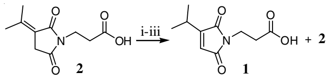
Scheme-I: Reagents, conditions and yields: (i) Aq. LiOH, THF, 0 °C to RT, 5 h (ii) Cyanuric chloride, Et 3 N, DCM, 0 °C to room temperature, 8 h (iii) Acetic acid, reflux, 5 h (three steps) 33 %
