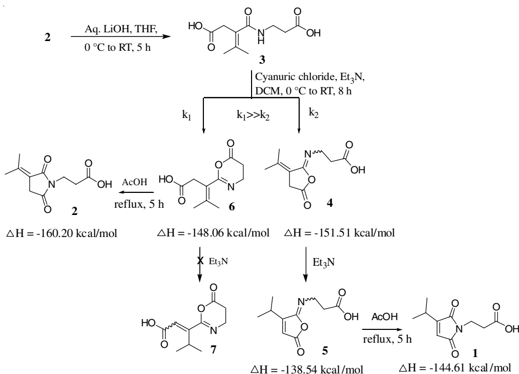
Fig. 1. Plausible reaction path for the formation of farinomalein ( 1 ) and isofarinomalein ( 2 )
