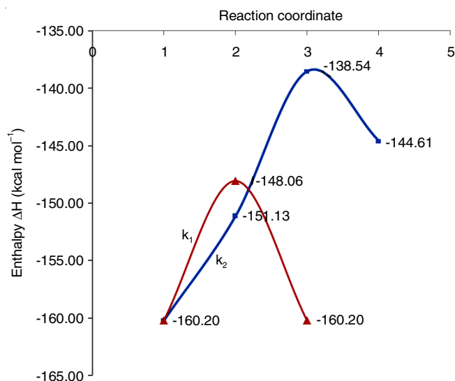
Fig. 2. Graph of enthalpy vs. reaction coordinate
