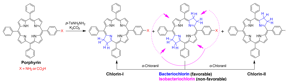
Figure 1. Possible formation of corresponding reduced isomers of TPC N1 and TPC C1 after diimide reduction of porphyrins TPP N1 and TPC C1 .
