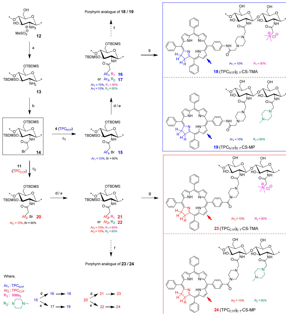
Scheme 2. Synthesis of TPC NIP -chitosan ( 18 , 19 ) and TPC CIP -chitosan ( 23 , 24 ) Nano-conjugates
