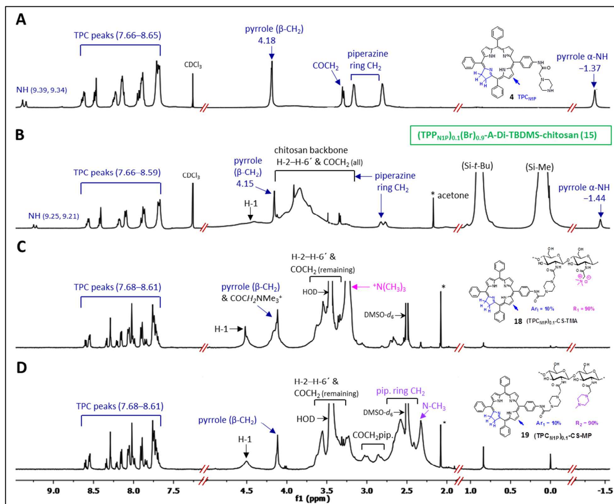
Figure 3. ^1\text{H} NMR spectra overlay of the main intermediate compounds and the final \text{TPC}_{\text{NIP}} -chitosan conjugates: (A) 4 ( \text{TPC}_{\text{NIP}} ); (B) 15 [ (\text{TPC}_{\text{NIP}})_{0.1}(\text{Br})_{0.9}\text{-A-Di-TBDMS-chitosan} ]; (C) 18 [ (\text{TPC}_{\text{NIP}})_{0.1}\text{-CS-TMA} ]; (D) 19 [ (\text{TPC}_{\text{NIP}})_{0.1}\text{-CS-MP} ].
