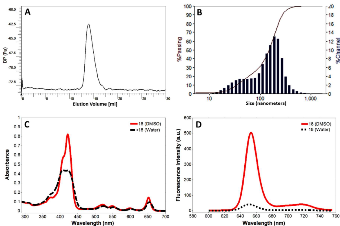
Figure 5. Photophysical results of representative TPC-chitosan nano-conjugate ( 18 ): (A) GPC chromatogram of viscosity measurement; (B) DLS measurement showing intensity wise particle size distribution; (C) Absorption spectra of 18 in DMSO and water at equal concentrations (0.3 mg/L); (D) Fluorescence emission spectra of 18 in DMSO and water [absorbance adjusted to 0.4 (1 cm path length) for both, and slit width used = 10 for both entrance and exit, \lambda_{\text{ex}} = 420 ].
