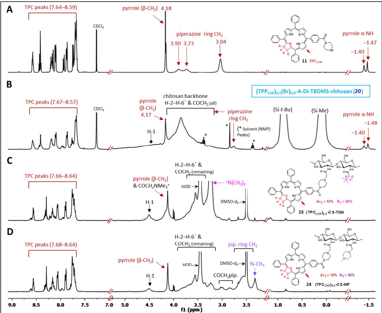
Figure 4. 1 H NMR spectra overlay of the main intermediate compounds and the final TPC CIP -chitosan conjugates: (A) 11 (TPC CIP ); (B) 20 [(TPC CIP ) 0.1 (Br) 0.9 -A-Di-TBDMS-chitosan]; (C) 23 [(TPC CIP ) 0.1 -CS-TMA]; (D) 24 [(TPC CIP ) 0.1 -CS-MP].
