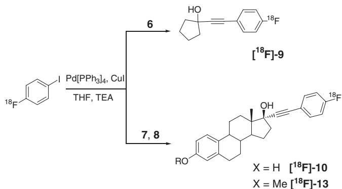
Figure 5. Sonogashira cross-coupling with 4- [^{18}\text{F}] fluoroiodobenzene
