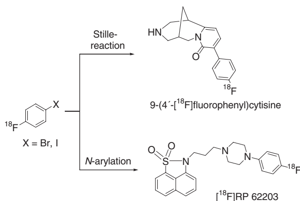
Figure 1. Cross-coupling reactions with 4- ^{18}\text{F} fluorohalobenzenes
