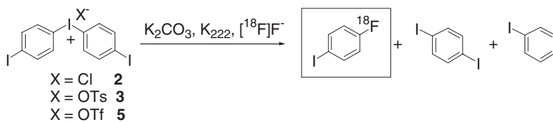
Figure 4. Radiosynthesis of 4-[ 18 F]fluoroiodobenzene
