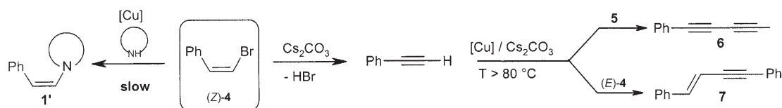
Scheme 3. Formation of by-products derived from ( Z )- \beta -bromostyrene (( Z )-4).
