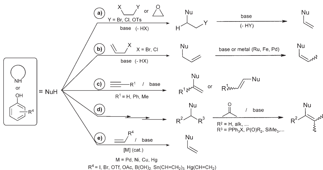
Scheme 2. Main routes to form N -vinylazoles and vinyl aryl ethers. Nu = nucleophile, Tf = trifluoromethanesulfonyl, Ts = toluene-4-sulfonyl.
