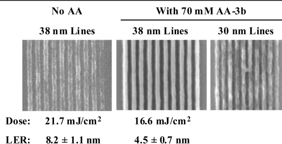
Figure 3. Scanning electron micrographs of dense line images printed using a control resist formulation with and without 70 mM 3b . 12
