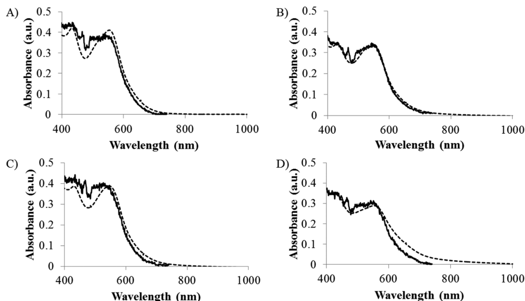
Figure 6. Overlaid absorption (dashed line) and excitation (solid line) spectra of (A) 1b , (B) 2b , (C) 1a , and (D) 2a in deoxygenated CH 3 CN at RT.
