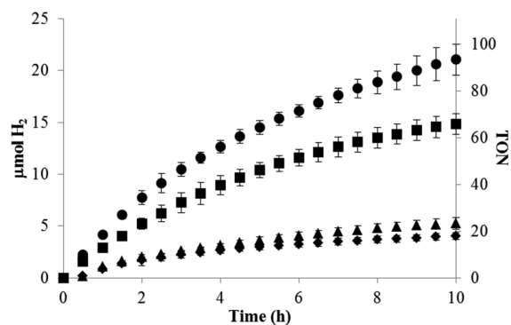
Figure 7. Hydrogen production profiles for photolysis systems with 2a (circles), 4a (squares), 1a (triangles), and 3a (diamonds). Photolysis systems contained 50 μM tetrametallic complex, 0.62 M H 2 O, 1.5 M DMA, and 110 μM [DMAH + ][CF 3 SO 3 − ] in deoxygenated CH 3 CN and irradiated at 470 nm. TON = mol H 2 /mol catalyst.
