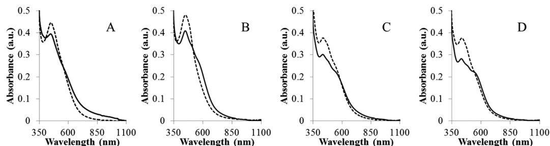
Figure 8. Electronic absorption spectroscopy after 10 h of photolysis in CH 3 CN in the presence of 1.5 M DMA, 0.62 M H 2 O, 110 \mu\text{M} [DMAH + ][CF 3 SO 3 - ] and (A) 50 \mu\text{M} 2a (solid line) or 50 \mu\text{M} 2b and 50 \mu\text{M} cis -[PtCl 2 (DMSO) 2 ] (dashed line), (B) 50 \mu\text{M} 1a (solid line) or 50 \mu\text{M} 1b and 50 \mu\text{M} cis -[PtCl 2 (DMSO) 2 ] (dashed line), (C) 50 \mu\text{M} 4a (solid line) or 50 \mu\text{M} 4b and 50 \mu\text{M} cis -[PtCl 2 (DMSO) 2 ] (dashed line), and (D) 50 \mu\text{M} 3a (solid line) or 50 \mu\text{M} 3b and 50 \mu\text{M} cis -[PtCl 2 (DMSO) 2 ] (dashed line).
