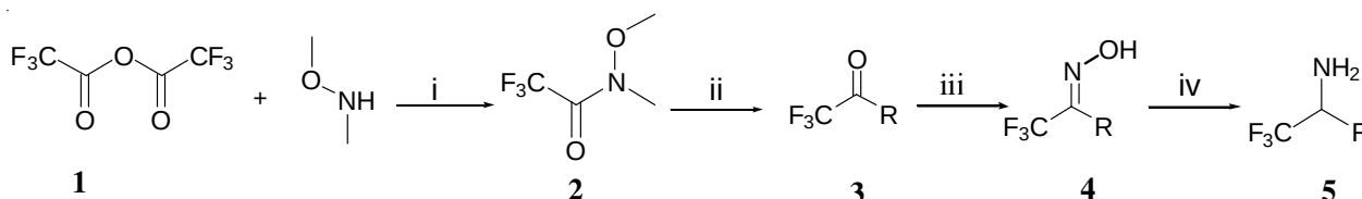
Scheme-I: Processes for synthesis of \alpha -trifluoromethylated amines starting from trifluoroacetic anhydride and conditions: (i) \text{CH}_2\text{Cl}_2 , rt, 95 %; (ii) \text{RMgBr} , THF, 0^\circ\text{C} , 76-90 %; (iii) \text{NH}_2\text{OH}\cdot\text{HCl} , \text{CH}_3\text{COONa} , rt, 90-99 %; (iv) \text{H}_2 , Raney nickel, 90^\circ\text{C} , 98 %
