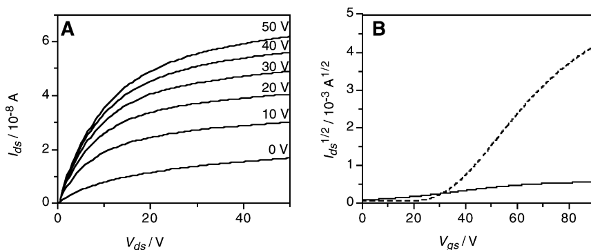
Figure 5. I/V characterization of OFET device B prepared using 2 . (A) I_{ds}/V_{ds} at different V_{gs} . (B) Corresponding plot of I_{ds}^{1/2} at saturation versus V_{gs} for 1 (device B, solid line) and for C_{60} (device A, dashed line).
