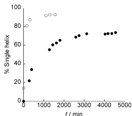
Figure 8. Time trace of duplex dissociation of 2 mM solutions of 11a (white circles) and 13a (black circles) in [\text{D}_5]\text{pyridine} monitored by ^1\text{H} NMR at 20^\circ\text{C} . The initial state is a freshly dissolved crystalline double helix.
