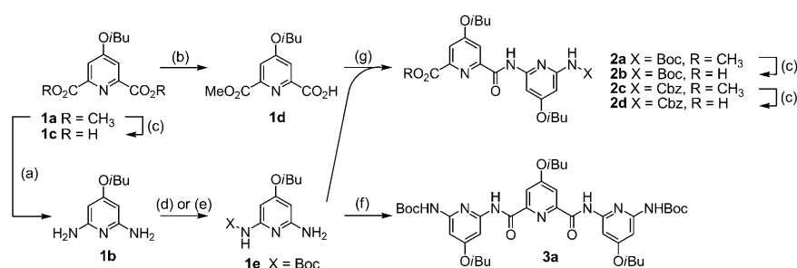
Scheme 1. a) I -NH 3 gas, MeOH, 1 h, RT; 2- KOH, Br 2 , dioxane, 0°C for 10 min then 25°C for 30 min and 70°C for 1.5 h, 78% yield; b) NaOH, MeOH/dioxane, 2 h, 25°C, 72% yield; c) NaOH, MeOH/dioxane/water, 2 h, RT, 95% yield; d) lithium bis(trimethylsilyl)amide, di- tert -butyldicarbonate, THF, 3.5 h, RT, 52% yield; e) lithium bis(trimethylsilyl)amide, benzyl chloroformate, THF, 3.5 h, RT, 56% yield; f) I - 1c , SOCl 2 , 30 min, reflux; 2- 1e , DIEA, THF; 12 h., 25°C, 75% yield; g) I - 1d , SOCl 2 , 30 min, reflux 2- 1e , DIEA, THF, 12 h., 25°C, 81% yield for 2a ; I - 1d , oxalyl chloride, DMF, toluene, 2 h, RT; 2- 1f , DIEA, THF, 12 h, RT, 98% for 2c .
