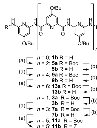
Scheme 2. a) 2b or 2d , 1-chloro- N,N ,2-trimethylpropenylamine, CH 2 Cl 2 , then DIEA, CH 2 Cl 2 ; b) TFA, CH 2 Cl 2 .
