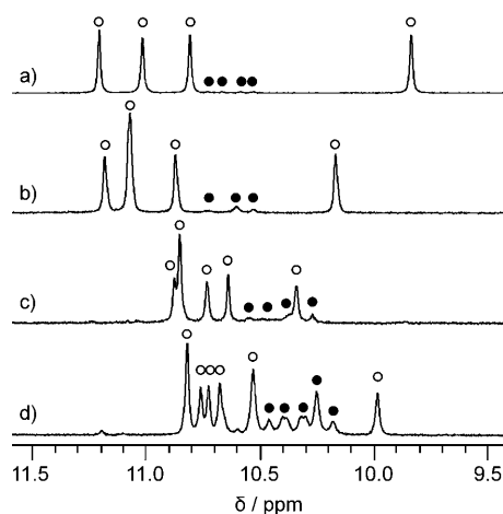
Figure 7. Part of the 300 MHz ^1\text{H} NMR spectra at 20^\circ\text{C} of 2 mM [\text{D}_5]\text{pyridine} solutions showing the amide resonances of: a) 7a ; b) 9a ; c) 11a and d) 13a at equilibrium. Signals belonging to the single and double helix are respectively marked with white and black circles.
