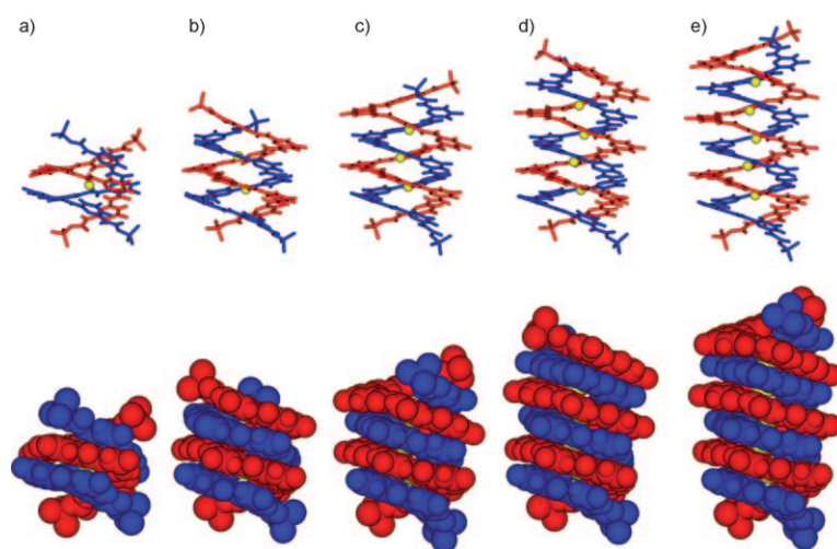
Figure 1. Side view of the solid-state structures in stick (top) and CPK (bottom) representations of: a) pentamer 5a ; b) heptamer 7a ; c) nonamer 9a ; d) undecamer 11a ; e) tridecamer 13a . The two strands of the double helices are shown as red and blue and water molecules as yellow sticks. Isobutoxy side chains, hydrogen atoms and solvent molecules (except water included in the channel) have been omitted for clarity. All helices are displayed in the same orientation, as illustrated by the identical appearance of their lower part.
