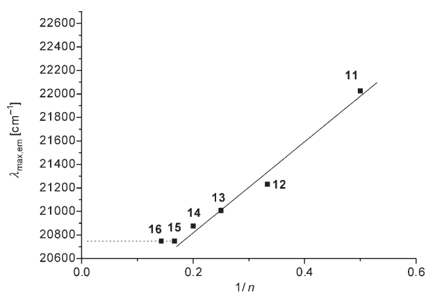
Figure 5. Correlation of the emission maxima \lambda_{\max,em} and phenothiazine units n for 11–14 (solid line: \lambda_{\max,em} = 3876 \cdot 1/n + 20042 ( r^2 = 0.980 )); dotted line: effective conjugation length at 482 nm).
