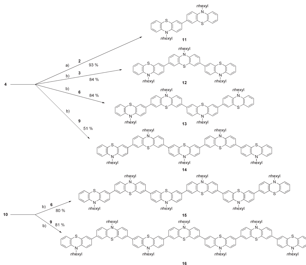
Scheme 2. Synthesis of oligophenothiazines: a) 5 mol % [\text{Pd}(\text{PPh}_3)_4] , \text{K}_2\text{CO}_3 , 1,4-dioxane/ \text{H}_2\text{O} 2:1, 90^\circ\text{C} , 2 d; b) 5 mol % [\text{Pd}(\text{PPh}_3)_4] , \text{K}_2\text{CO}_3 , DME/ \text{H}_2\text{O} 2:1, 85^\circ\text{C} , 18 h.
