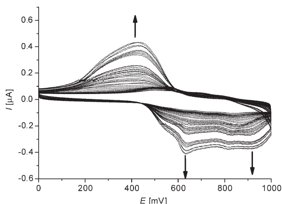
Figure 7. Multisweep experiment with tetramer 13 upon dropwise increase of concentration from 10^{-5} to 10^{-4}\text{ M} ( \text{CH}_2\text{Cl}_2 ; T=293\text{ K} ; electrolyte: 0.05\text{ M NBu}_4\text{PF}_6 ( \text{CH}_2\text{Cl}_2 ); \nu=250\text{ mV s}^{-1} ; Pt as a working electrode, Ag/AgCl as a reference electrode, and Pt as a counter electrode (determined vs. ferrocene, E_0^{0/+1}=+450\text{ mV} ).
