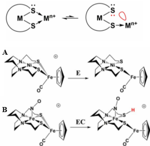
Figure 1. Hemilability in MN_2S_2 bridging thiolates. 17
