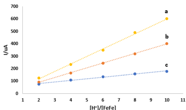
Figure 8. Dependence of current heights of electrocatalytic waves on acid concentration. (a) 1 ( -1.48 V), (b) (\mu\text{-pdt})[\text{Fe}(\text{CO})_3][\text{Fe}(\text{CO})_2\text{PPh}_3] ( -1.73 V), (c) (\mu\text{-pdt})[\text{Fe}(\text{CO})_3]_2 ( -1.95 V).
