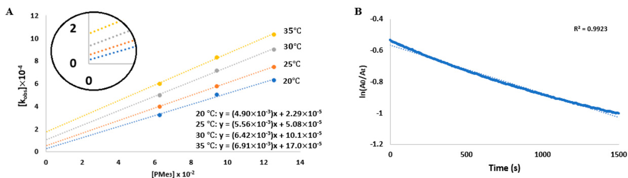
Figure 12. (a) Plots of k_{\text{obs}} vs [\text{PMe}_3] for the formation of 1\text{-PMe}_3 from 1 measured at 20/25/30/35 °C (conditions: SI Table S4, entries 1–12). (b) Example plot of \ln(A_0/A_t) vs time over four half-lives (conditions: SI Table S4, entry 1).
