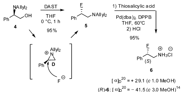
Scheme 3. Rearrangement of 4
