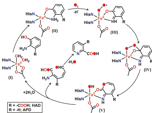
Scheme 2. Proposed Catalytic Cycle of 2-Aminophenol Dioxygenases
