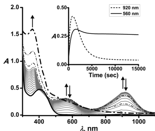
Figure 3. Time-dependent optical spectral changes during the reaction of 2 ·ClO 4 with dioxygen at 298 K (concentration: 0.5 mM in acetonitrile).
