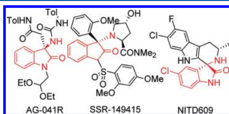
Figure 1. Selected bioactive quaternary aminooxindoles.
