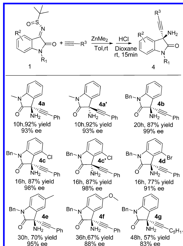
Scheme 2. Alkynylation of Various Ketimines a
