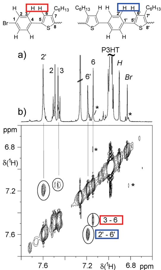
Figure 1. (a) ^1\text{H} NMR spectrum (region) of a P3HT obtained upon Kumada catalyst-transfer polymerization of 1 initiated by 4 at RT and (b) the corresponding region from the ROESY spectrum. Br and H, thiophene signals from Br and H chain termination; *, ^{13}\text{C} satellites of the P3HT backbone signal.
