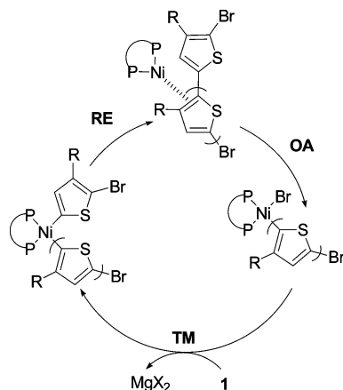
Scheme 1. State-of-the-Art Vision of the Mechanism of Chain-Growth KCTP 16
