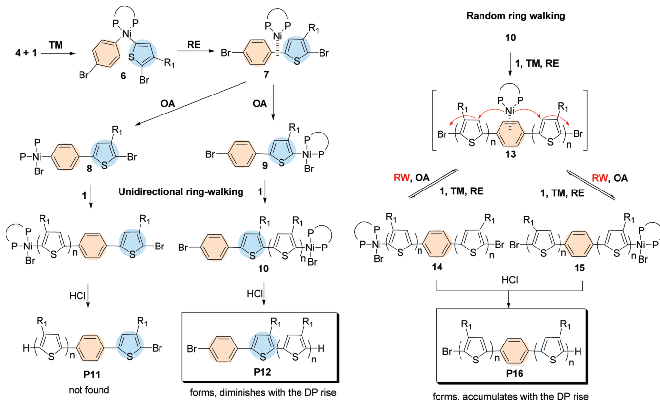
Scheme 4. Unidirectional versus Random Catalyst Walking upon KCTP
