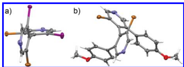
Figure 1. ORTEP plots of one of the four molecules within the asymmetric units of (a) 3 and (b) 4b . Thermal ellipsoids set at 50% probability and hydrogen atoms shown as sticks. The absolute configurations are P for 3 and M for 4b .
