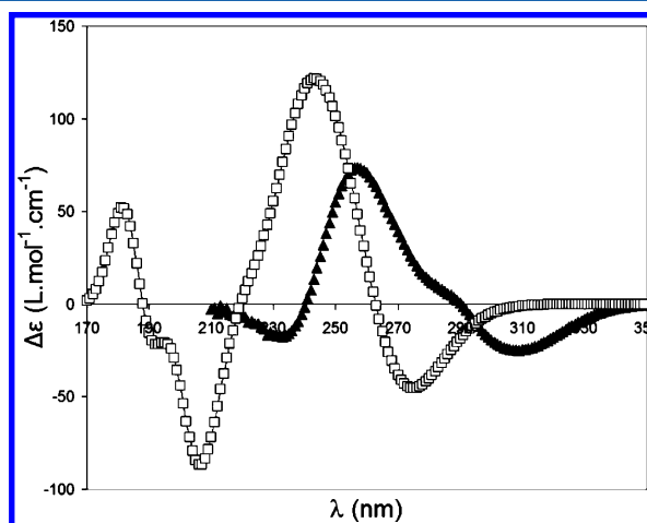
Figure 3. Comparison of experimental (black triangles) and theoretical (squares) ECD spectra for the ( M )- 4b enantiomer.
