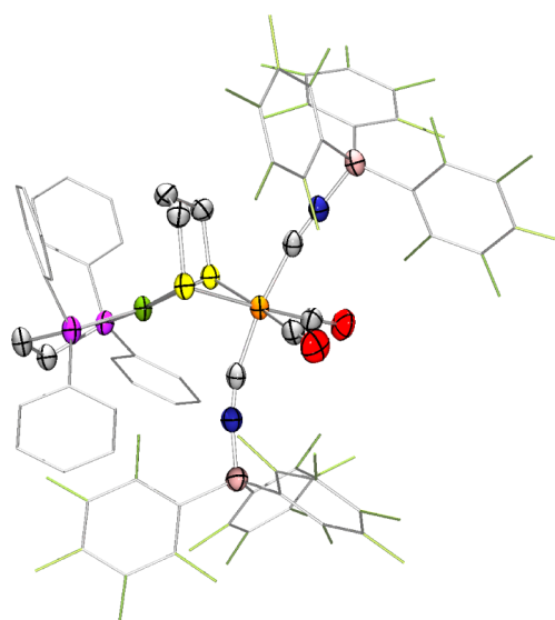
Figure 2. Structure of [(CO) 2 (CNBAr F 3 ) 2 Fe(pdt)Ni(dppe)], 1 (BAr F 3 ) 2 , with ellipsoids shown at 50% probability and with H atoms omitted for clarity. Phenyl and pentafluorophenyl groups are de-emphasized for clarity.
