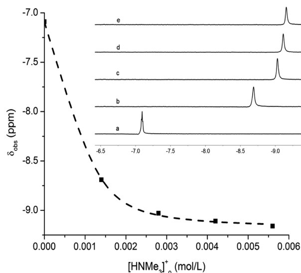
Figure 4. ^1\text{H} NMR chemical shift for \text{Et}_4\text{N}[\text{H3}(\text{BAR}^{\text{F}_3})_2] upon titration with \text{HNMe}_3[\text{BAR}^{\text{F}_3}] in \text{CD}_2\text{Cl}_2 ( 20^\circ\text{C} ). Inset: ^1\text{H} NMR (500 MHz) spectra of the titration of \text{Et}_4\text{N}[\text{H3}(\text{BAR}^{\text{F}_3})_2] with \text{HNMe}_3[\text{BAR}^{\text{F}_3}] in \text{CD}_2\text{Cl}_2 ( 20^\circ\text{C} ): (a) 0, (b) 1.0, (c) 2.0, (d) 3.0, and (e) 4.0 equiv.
