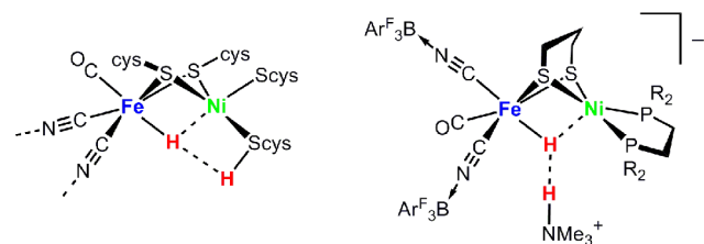
Figure 5. Dihydrogen bonding in [\text{H}_3(\text{BAr}^{\text{F}_3})_2]^- and the analogous interaction proposed for Ni–R.
