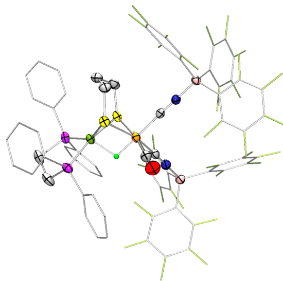
Figure 3. Structure of the anion in \text{Et}_4\text{N}[(\text{CO})(\text{CNBAr}^{\text{F}}_3)_2\text{Fe}(\text{H})(\text{pdt})\text{Ni}(\text{dppe})]^- , \text{Et}_4\text{N}[\text{H}3(\text{BAr}^{\text{F}}_3)_2] , with ellipsoids shown at 50% probability and H atoms except for the bridging hydride omitted. Phenyl and pentafluorophenyl groups are de-emphasized for clarity.
