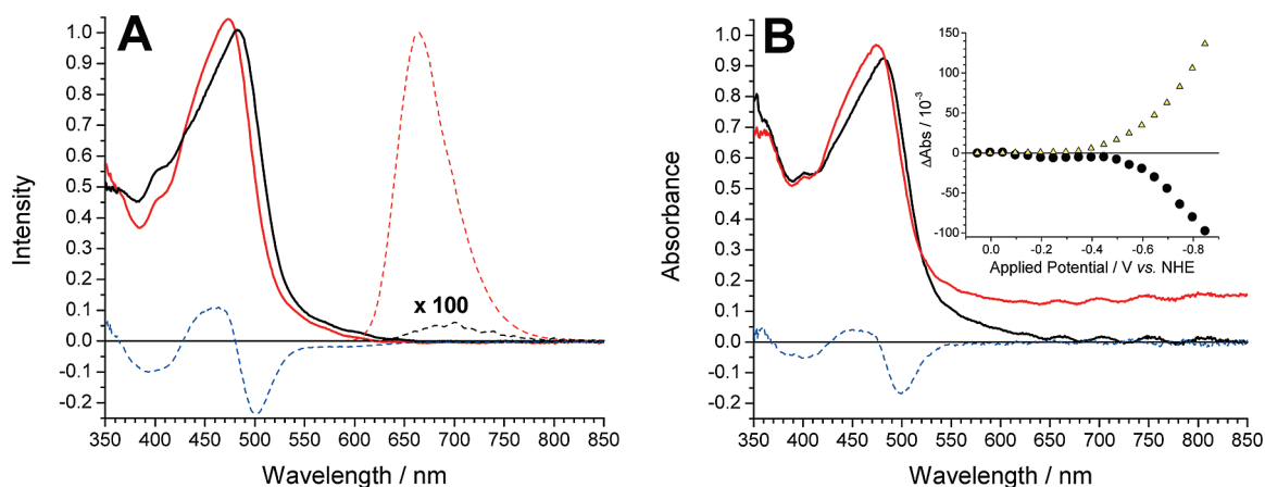
Figure 1. (A) Absorption and photoluminescence spectra of [\text{Ru}(\text{dtbbpy})_2(\text{dcb})]^{2+} anchored to a \text{TiO}_2 thin film immersed in 100 mM \text{LiClO}_4/\text{CH}_3\text{CN} (black); in neat acetonitrile after removal of the \text{LiClO}_4/\text{CH}_3\text{CN} solution and 10 acetonitrile washings (red); their difference spectrum (blue, dashed). (B) Absorption spectrum of [\text{Ru}(\text{dtbbpy})_2(\text{dcb})]^{2+} anchored to a \text{TiO}_2/\text{FTO} thin film electrode in 100 mM \text{LiClO}_4/\text{CH}_3\text{CN} with 500 mM \text{TBAClO}_4 at open circuit (black) and biased to -0.85 V vs NHE (red); their difference spectrum corrected for the absorbance features due to \text{TiO}_2(\text{e}^-) s (blue, dashed). Inset: absorbance changes measured as a function of applied bias for the maximum bleach at 500 nm (circles) and \text{TiO}_2(\text{e}^-) s at 750 nm (open triangles). The bias was held at each potential for 1–2 min before each steady-state absorption measurement.
