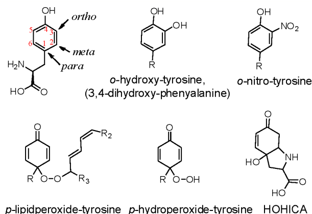
Figure 1. Tyrosine structure showing the different ring positions and different products of tyrosine oxidation involving modifications at the ortho and para positions.
