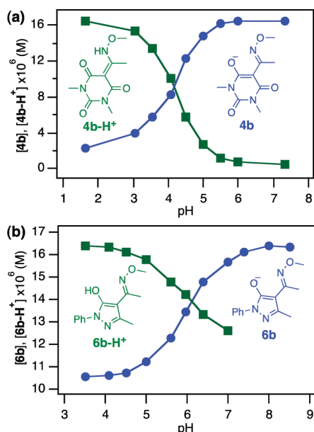
Figure 3. Plot of the concentration of (a) 4b , 4b-H + , and (b) 6b , 6b-H + as a function of pH. In (a), the green squares represent 4b-H + ( \lambda_{\text{max}} = 298 nm), and blue circles represent carbanion 4b ( \lambda_{\text{max}} = 261 nm). In (b), the green squares represent 6b-H + ( \lambda_{\text{max}} = 270 nm), where the last three data points were omitted due to spectral overlap, and the blue circles represent carbanion 6b ( \lambda_{\text{max}} = 253 nm). See SI for representative UV-vis spectra of 4b and 6b at high and low pH.
