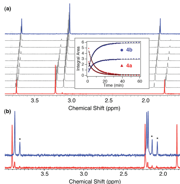
Figure 2. 1 H NMR analysis of the decomposition of (a) 4a to 4b and (b) 6a to 6b in 10% D 2 O, PBS, pH 7.4 at room temperature. In each case, the red spectrum was collected at the start of the experiment, and the blue spectrum after complete decomposition. In the insert of (a), the kinetics of decomposition are shown. The red triangles represent the N-CH 3 's (6H) and the oxime C-CH 3 (3H) of 4a, and the blue circles represent the N-CH 3 's (6H) and the oxime C-CH 3 (3H) of carbanion 4b. The solid curves are calculated best fits to a single exponential function ( k = 2.4 \times 10^{-3} \text{ s}^{-1} for each fit). In (b), the asterisks (*) indicate signals due to the minor anti -6b isomer.
