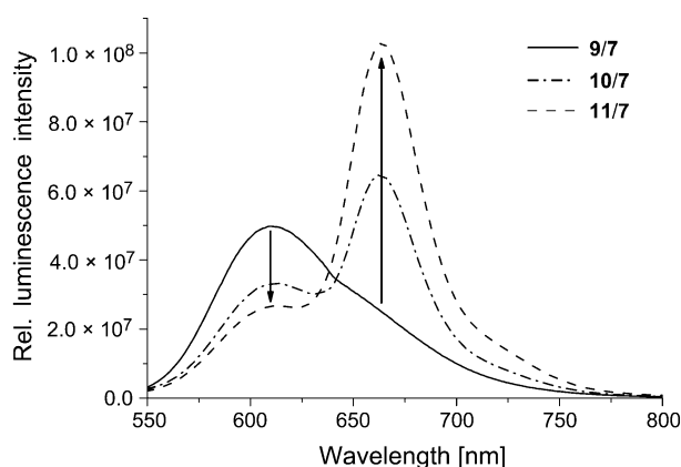
Fig. 6. Steady-state measurements ( \lambda_{\text{ex}} 430 nm) of the FRET pair Ru/Cy at different distances between them in hybridized DNA strands ( 9/7 : no Cy; 10/7 : Cy 2 ; 11/7 : Cy 1 )
