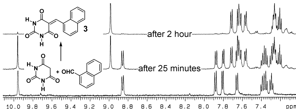
Figure 1. ^1\text{H} -NMR (500 MHz) reaction following for 1-naphthaldehyde (1 mM) condensation with barbituric acid (5 mM) in \text{CF}_3\text{COOH} .
