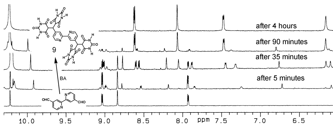
Figure 6. 1 H-NMR (500 MHz) following of barbituric acid (10 mM) condensation with 2,2'-bipyridine-4,4'-carboxaldehyde (2.5 mM) in TFA-DMSO (3:1) at room temperature.
