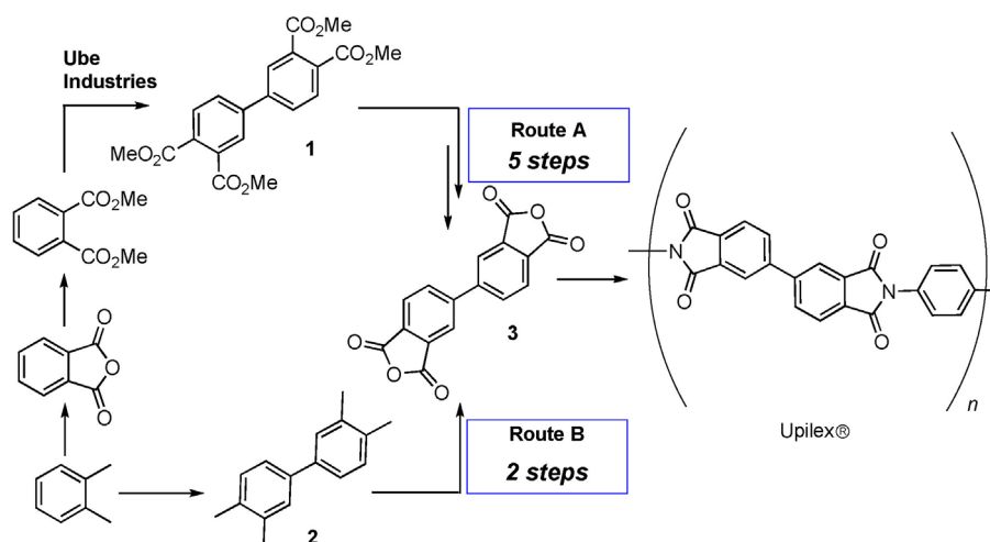
Scheme 1. Current and proposed alternative routes for the industrial synthesis of 4,4'-bipthalic anhydride.
