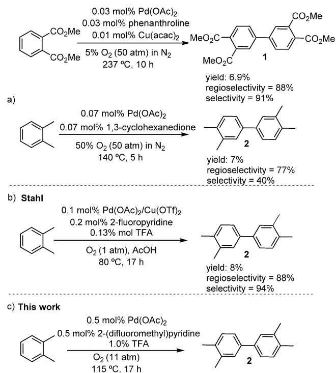
Scheme 2. Developed catalyst for the CDC of arenes towards the synthesis of 4,4'-bipthalic anhydride.
