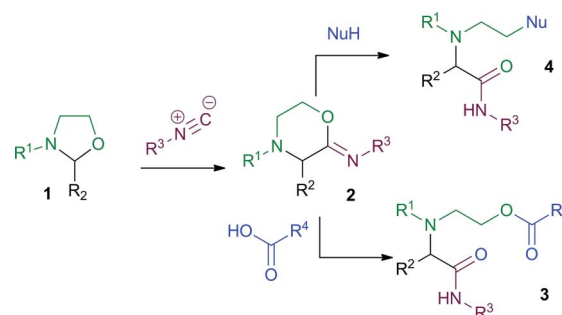
Scheme 2 3-CRs of 1,3-oxazolidines.
