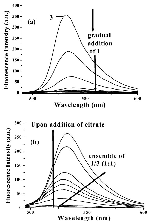
Fig. 9 (a) Change in emission of dye 3 ( c = 8.0 \times 10^{-5} \text{ M} ) upon increasing addition of 1 ( c = 4.2 \times 10^{-4} \text{ M} ) and (b) retrieval of emission upon increasing addition of citrate ( c = 4.62 \times 10^{-3} \text{ M} ) to the ensemble 1/3 in \text{CH}_3\text{CN}-\text{H}_2\text{O} (4 : 1, v/v, pH 6.3, 10 mM Tris/HCl buffer).
