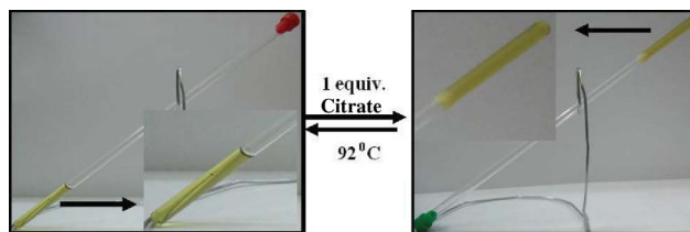
Fig. 12 Photographs showing phase changes for a gel of 2 ( c = 6.29 \times 10^{-3} M) with citrate in \text{CH}_3\text{CN} .
