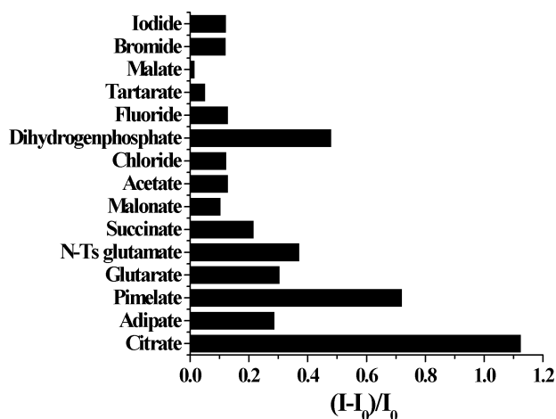
Fig. 3 Fluorescence ratio [(I - I_0)/I_0] of 2 ( c = 6.27 \times 10^{-5} M) at 385 nm upon addition of 10 equiv. of a particular anion in \text{CH}_3\text{CN}-\text{H}_2\text{O} (4:1 v/v, pH 6.3, 10 mM Tris HCl buffer).
