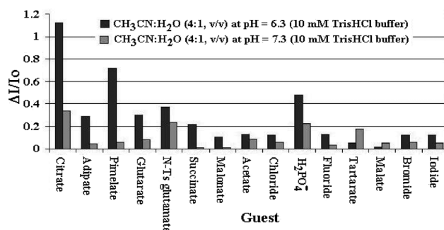
Fig. 5 Fluorescence ratio [(I - I_0)/I_0] of 2 ( c = 6.27 \times 10^{-5} M) at 385 nm upon addition of 10 equiv. of a particular anion in \text{CH}_3\text{CN}-\text{H}_2\text{O} (4:1 v/v 10 mM Tris HCl buffer) at pHs 6.3 and 7.3.
