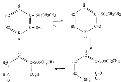
Figure 4. Isomerization of 2-hydroxypyridine 4 into 2-pyridone, which further could be hydrolyzed into low-molecular weight nontoxic products.
