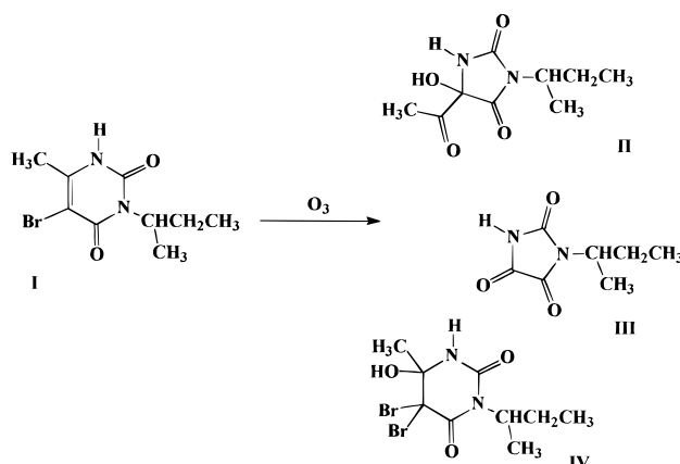
Figure 2. Products of bromacil ozonolysis.
