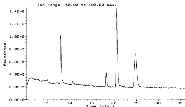
Figure 3. LC/MS total ion chromatogram of bromacil ozonolysis reaction mixture. Peaks at t_R = 7.9, 18.2, 20.6, and 24.8 min correspond to II , III , bromacil, and IV , respectively.
