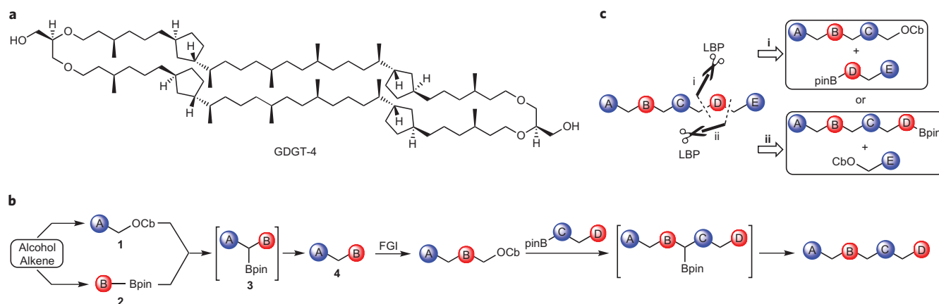
Figure 1 | Complex molecules with limited functionality present in nature and the potential traceless strategy for their synthesis. a , Structure of the GDGT membrane lipid of cosmopolitan pelagic Crenarchaeota. b , Lithiation-borylation-protodeboronation (LBP) strategy for the organic synthesis, showing the process for combining two fragments (A and B) followed by the removal of the boronic ester, and its repeated use (fragments C and D). c , Possible disconnections of a molecule using the traceless LBP strategy. Cb, N,N -diisopropyl carbamate; FGI, functional group interconversion.
