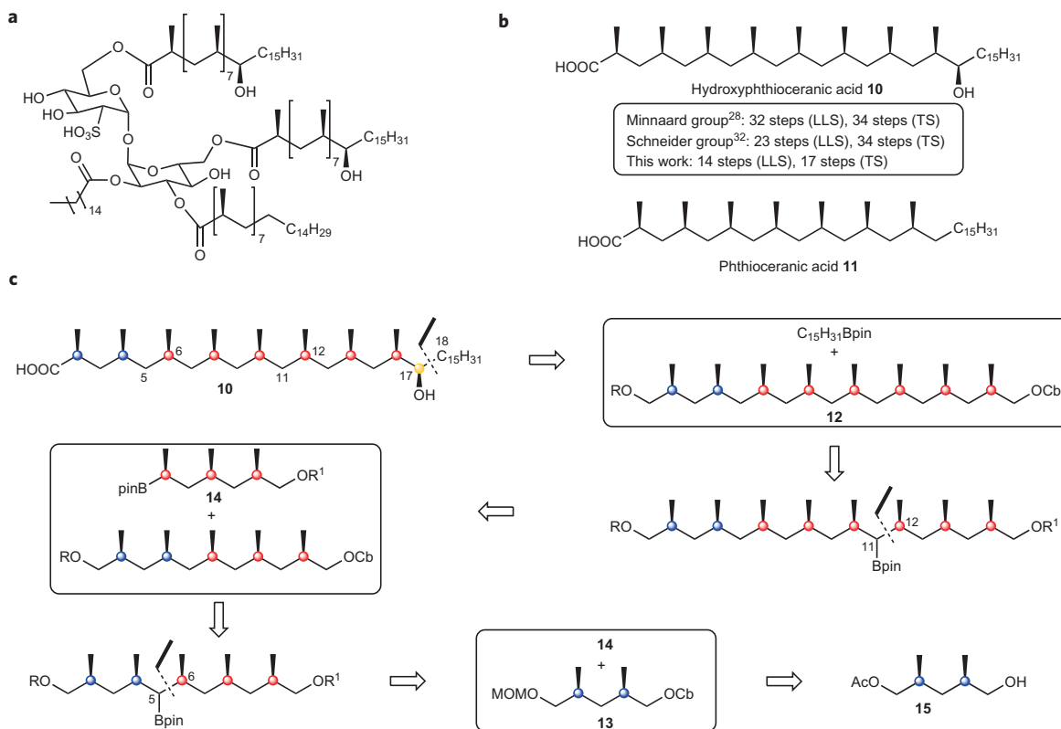
Figure 3 | Complex molecules of interest in this study associated with the cell-wall lipid of MTB. a , Structure of SL-1 the major cell-wall lipid of virulent human MTB. b , Structures of two polydeoxypropionates that are coupled to the sugar core of SL-1, hydroxyphthioceranic acid 10 and phthioceranic acid 11 . Syntheses of 10 have recently been reported by the Minnaard group 28 and by the Schneider group 32 . c , Retrosynthetic analysis of hydroxyphthioceranic acid 10 . This shows how we envisaged building the molecule from simpler fragments. LLS, longest linear sequence; TS, total number of steps.
