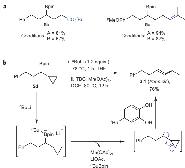
Figure 2 | Brief survey of the scope and mechanism of the protodeboronation reaction. a , Functional groups tested for compatibility with protodeboronation under two sets of conditions. Conditions A: n -BuLi, TBC, Mn(OAc) 3 ·2H 2 O, DCE, 12 h, 80 °C; Conditions B: TBAF, TBC, Mn(OAc) 3 ·2H 2 O, DCE, 12 h, 80 °C. b , Radical clock to probe the mechanism of the protodeboronation reaction. The formation of the ring-opened product indicates that protodeboronation occurs via a radical intermediate as shown.
