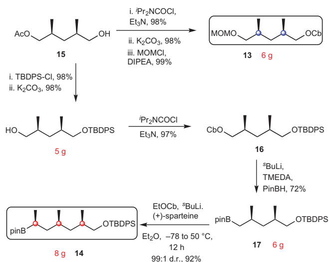
Figure 4 | Synthesis of building blocks 13 and 14 used in the synthesis of hydroxyphthioceranic acid 10 . DIPEA, N,N -diisopropylethylamine.
