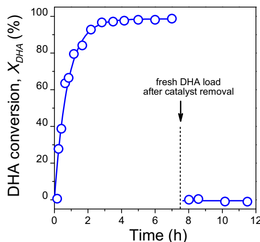
Fig. 1. DHA conversion ( X_{DHA} ) as a function of reaction time on 6.9SnAl. Catalyst removal at 7 h [353 K; ethanol/DHA = 43 (molar); 1 g of catalyst].
