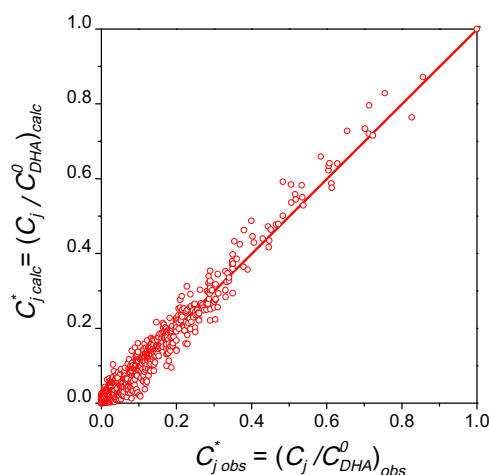
Fig. 7. Parity plot of the experimental ( C_j^* = (C_j/C_{DHA}^0)_{obs} ) and predicted ( C_j^* = (C_j/C_{DHA}^0)_{calc} ) relative concentrations of DHA and products.
