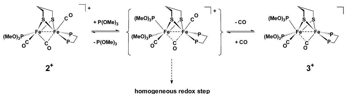
Scheme 9. Proposed Reaction Sequence for the Interconversion 2^+ \leftrightarrow 3^+ a
