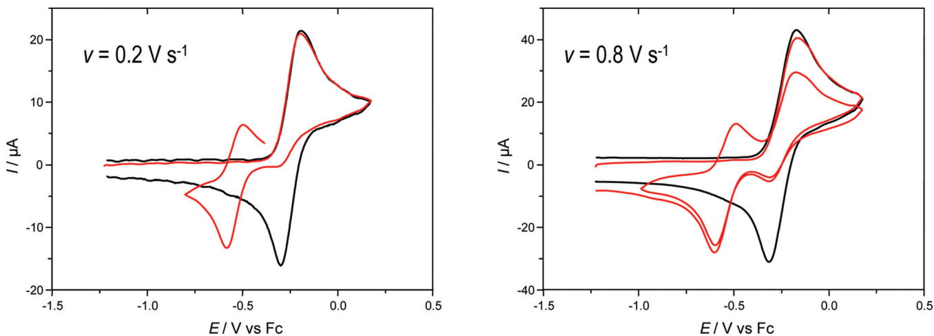
Figure 3. CV of [\text{Fe}_2(\text{CO})_4(\kappa^2\text{-dppe})(\mu\text{-pdt})] ( 1 ) (1.1 mM) in \text{CH}_2\text{Cl}_2\text{-}[\text{NBu}_4][\text{PF}_6] in the absence (black lines) and in the presence (red lines) of 1 equiv of \text{P}(\text{OMe})_3 (vitreous carbon electrode; potentials are in V vs \text{Fc}^+/\text{Fc} ).
