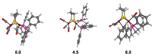
Figure 2. DFT optimized structures of relevant 1 + isomers. The energy (in kcal/mol) of each isomer, relative to the lowest-energy one, is shown below each structure. For the sake of clarity atoms are shown as follow. Carbon, gray; hydrogen, white; sulfur, yellow; oxygen, red; phosphorus, light purple; iron, dark purple.
