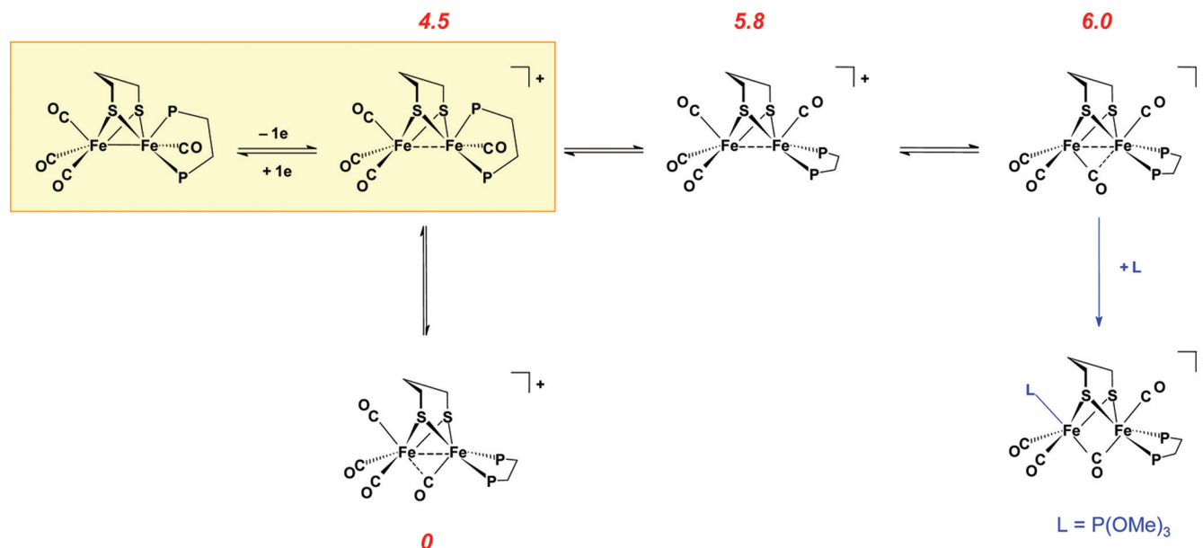
Scheme 8. Schematic Representation of the 1^+ Isomers That Can Be Formed upon One-Electron Oxidation of 1^a
