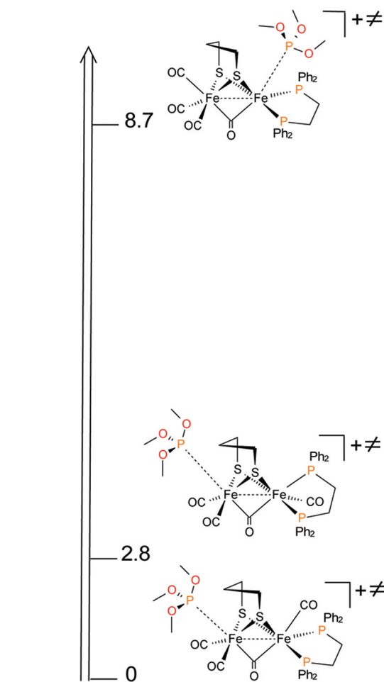
Scheme 5. Relative Energies a and Structures of the Transition States for the Reaction between 1^+ and P(OMe)_3
