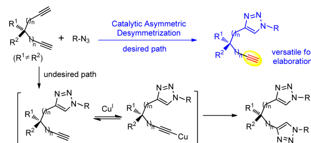
Scheme 1. Desymmetrization of Dialkynes by CuAAC
