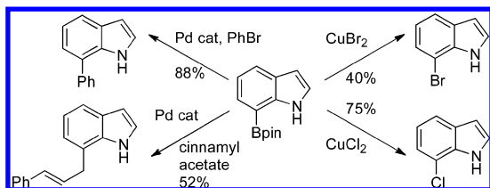
Scheme 2. Functionalization of 7-Borylindoles
