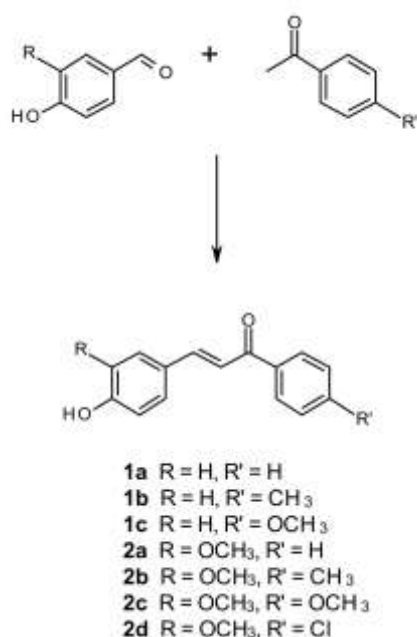
Scheme 2. Synthesis of chalcones 1a-1c and 2a-2d .
