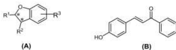
Figure 1. Structure of compounds (A) and (B)
