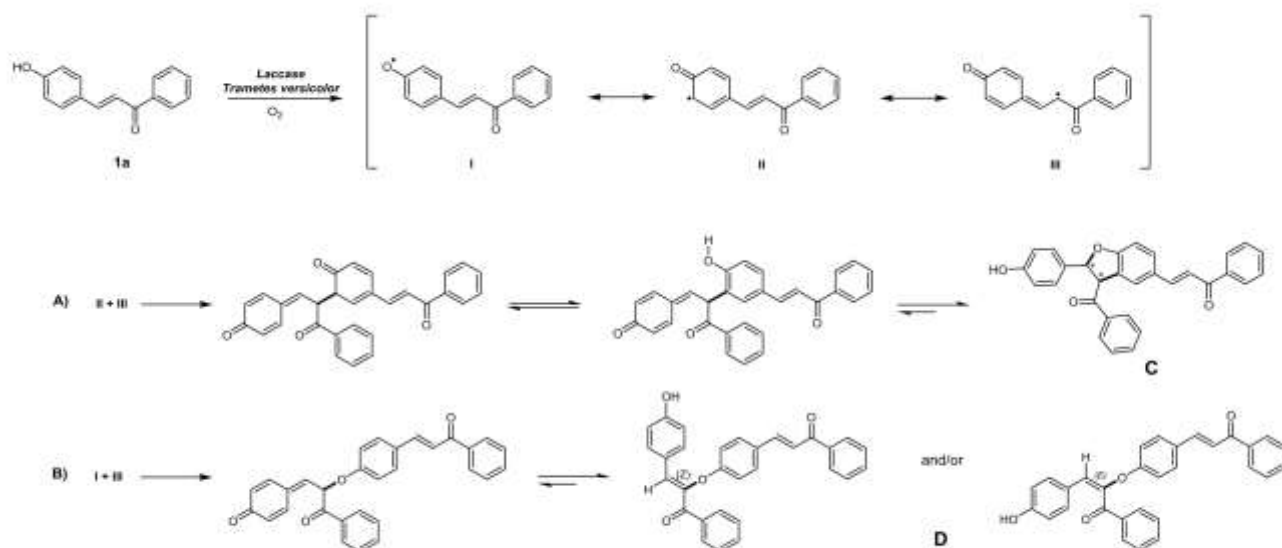
Scheme 3. Laccase-catalyzed dimerization of 4-hydroxy-chalcone 1a .
