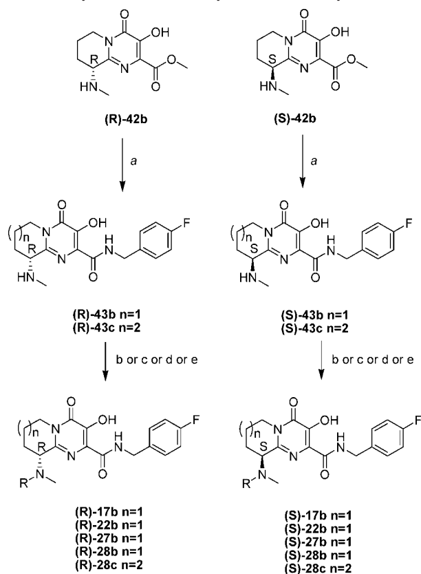
Scheme 3. Synthesis of Chiral Pyrimidinone Benzylamides a
