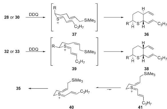
Scheme 6. Origins of Minor Products with Allylsilane Nucleophiles
