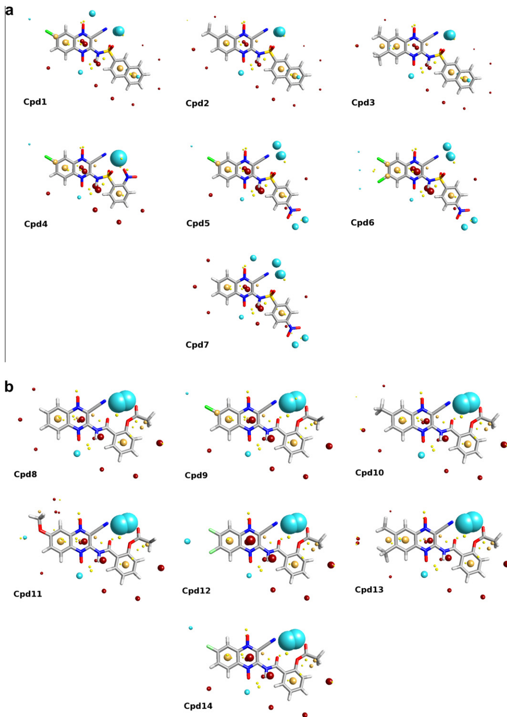
Figure 1. Graphical representation of the structure-activity relationship for sulfonamides (a) and acetoxybenzamides (b). Field Points are colored as follows: Blue; negative field points (like to interact with positives/H-bond donors on a protein), red; positive field points (like to interact with negatives/H-bond acceptors on a protein), yellow; van der Waals surface field points (describing possible surface/vdW interactions), gold/orange; Hydrophobic field points (describe regions with high polarizability/hydrophobicity).
